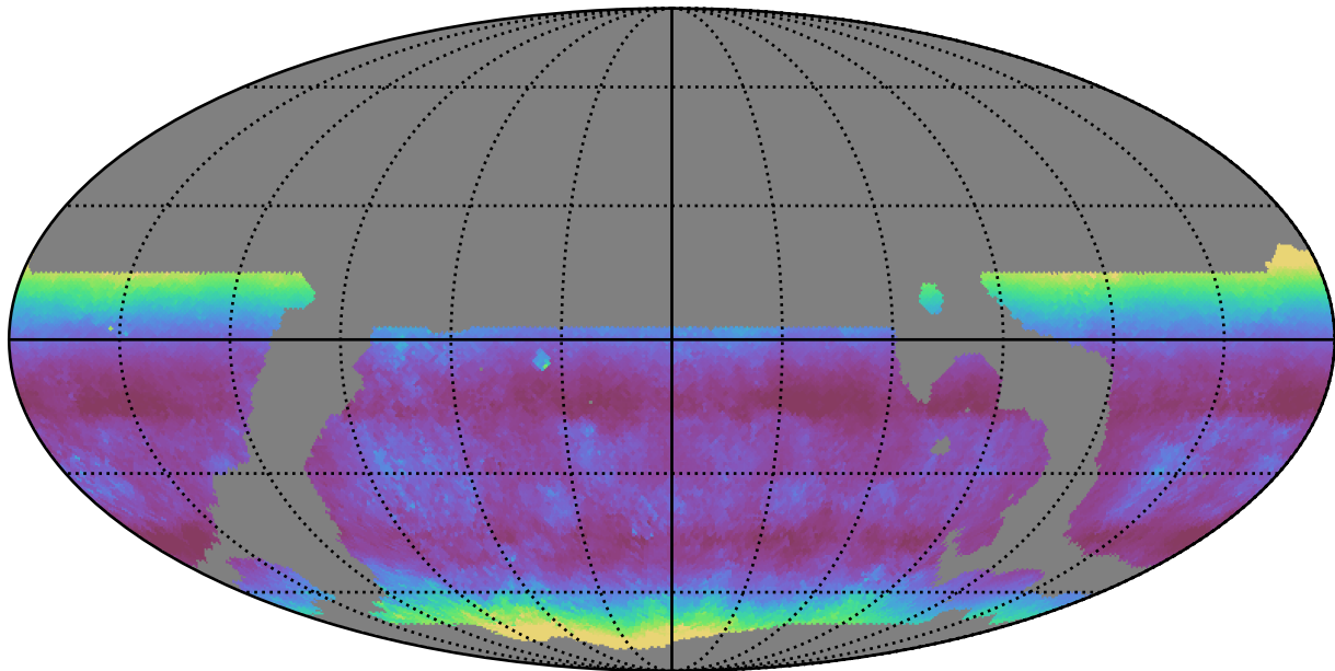
weather_cloudso4v3.4_10yrs WFD g band: Median airmass
