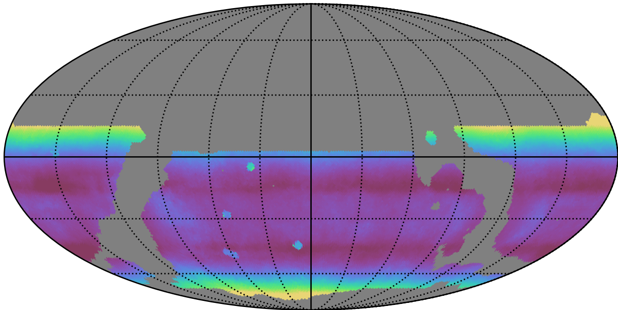
weather_cloudso4v3.4_10yrs WFD all bands: Median airmass
