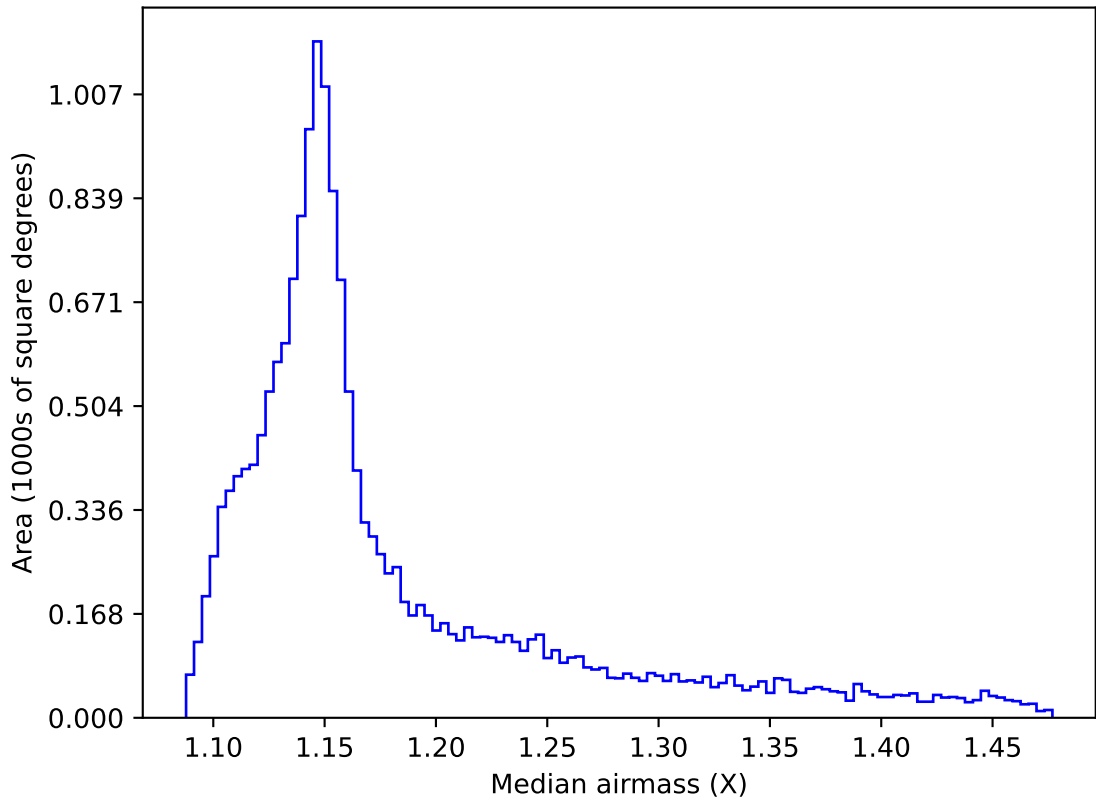
weather_cloudso4v3.4_10yrs WFD all bands: Median airmass
