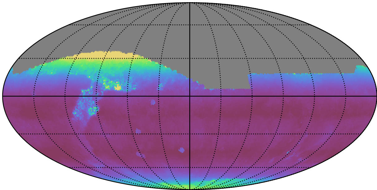
weather_cloudso4v3.4_10yrs All sky z band: Median airmass
