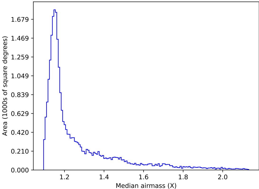
weather_cloudso4v3.4_10yrs All sky z band: Median airmass
