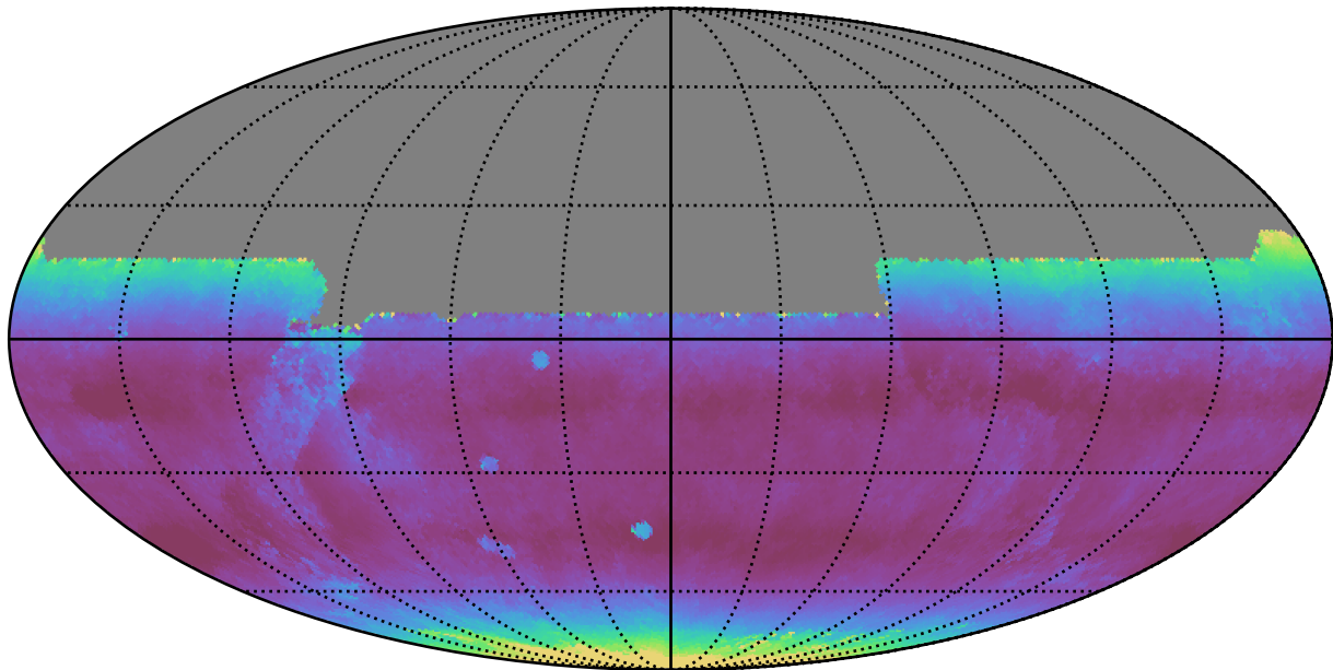
weather_cloudso4v3.4_10yrs All sky y band: Median airmass
