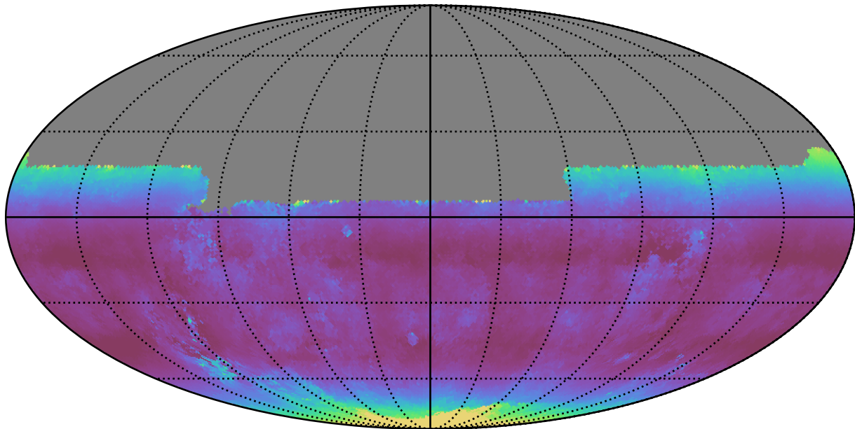
weather_cloudso4v3.4_10yrs All sky u band: Median airmass
