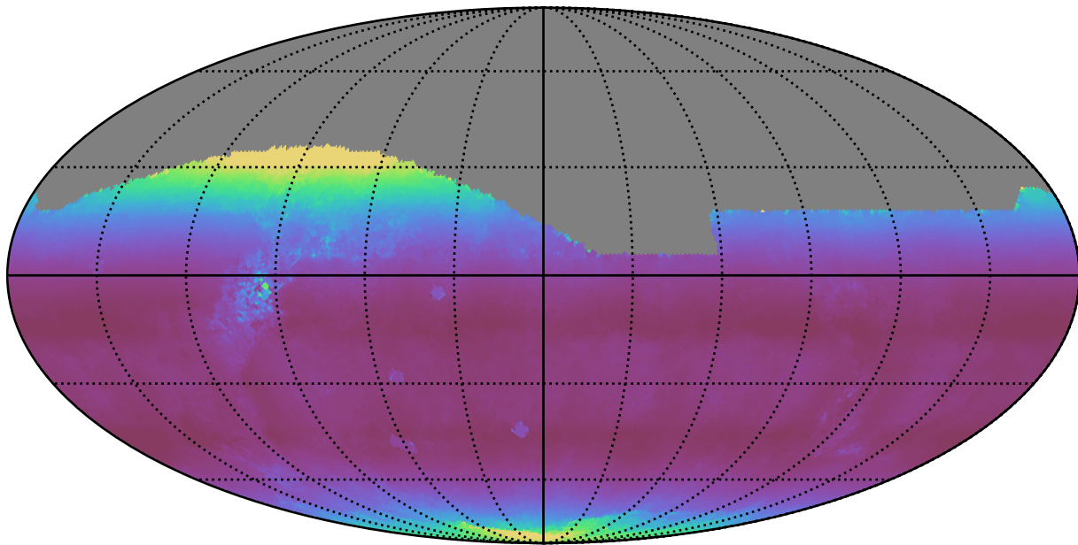
weather_cloudso4v3.4_10yrs All sky r band: Median airmass
