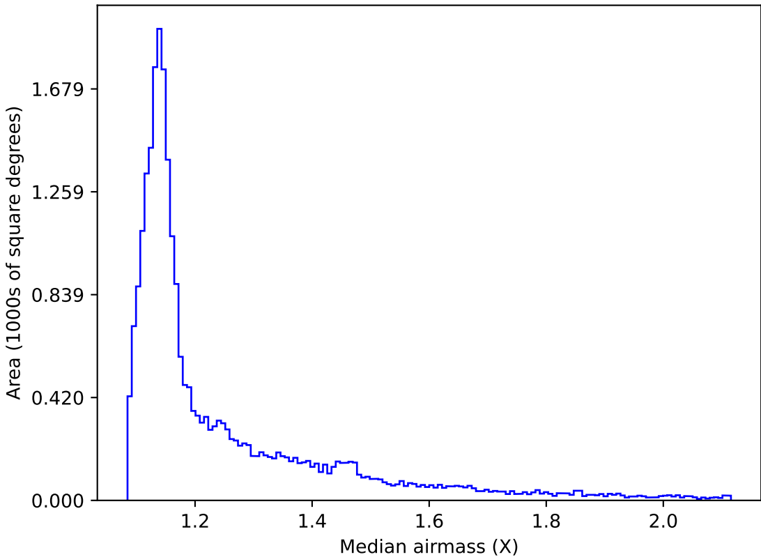
weather_cloudso4v3.4_10yrs All sky i band: Median airmass
