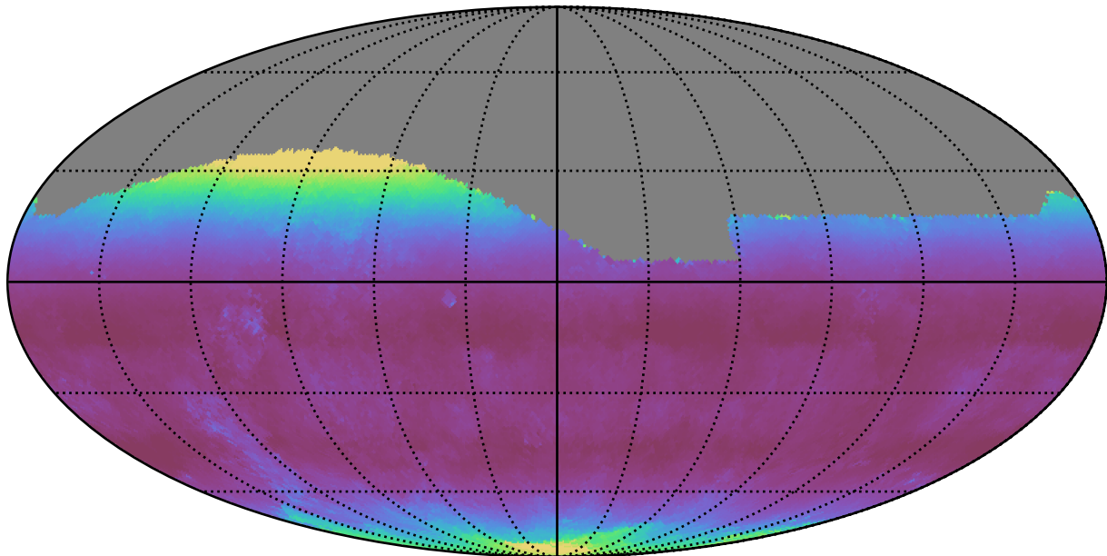
weather_cloudso4v3.4_10yrs All sky g band: Median airmass
