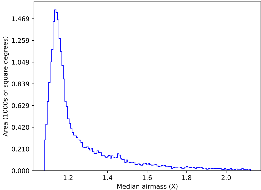
weather_cloudso4v3.4_10yrs All sky g band: Median airmass
