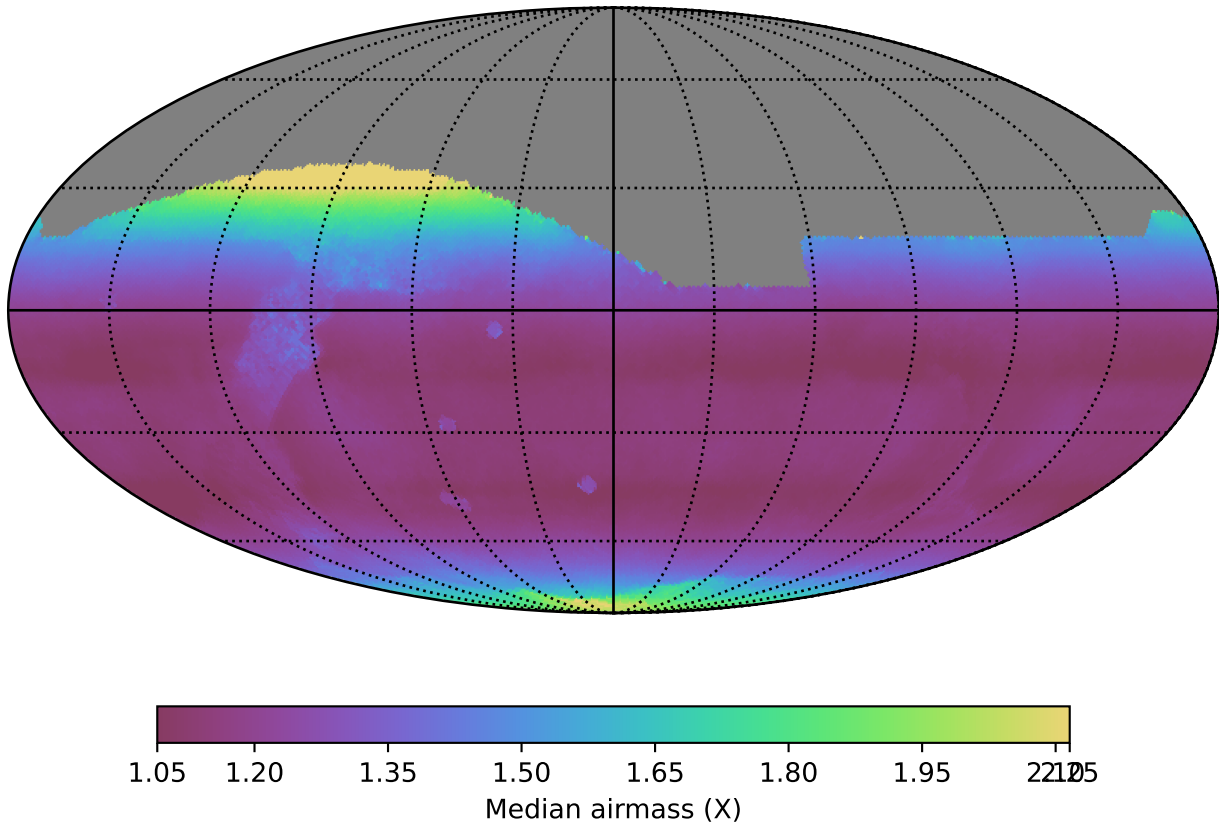
weather_cloudso4v3.4_10yrs All sky all bands: Median airmass
