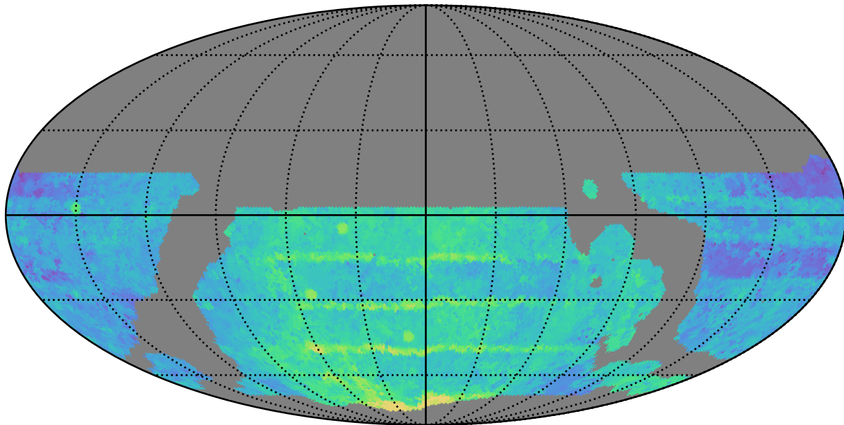
weather_cloudso4v3.4_10yrs WFD z band: Median Season Length
