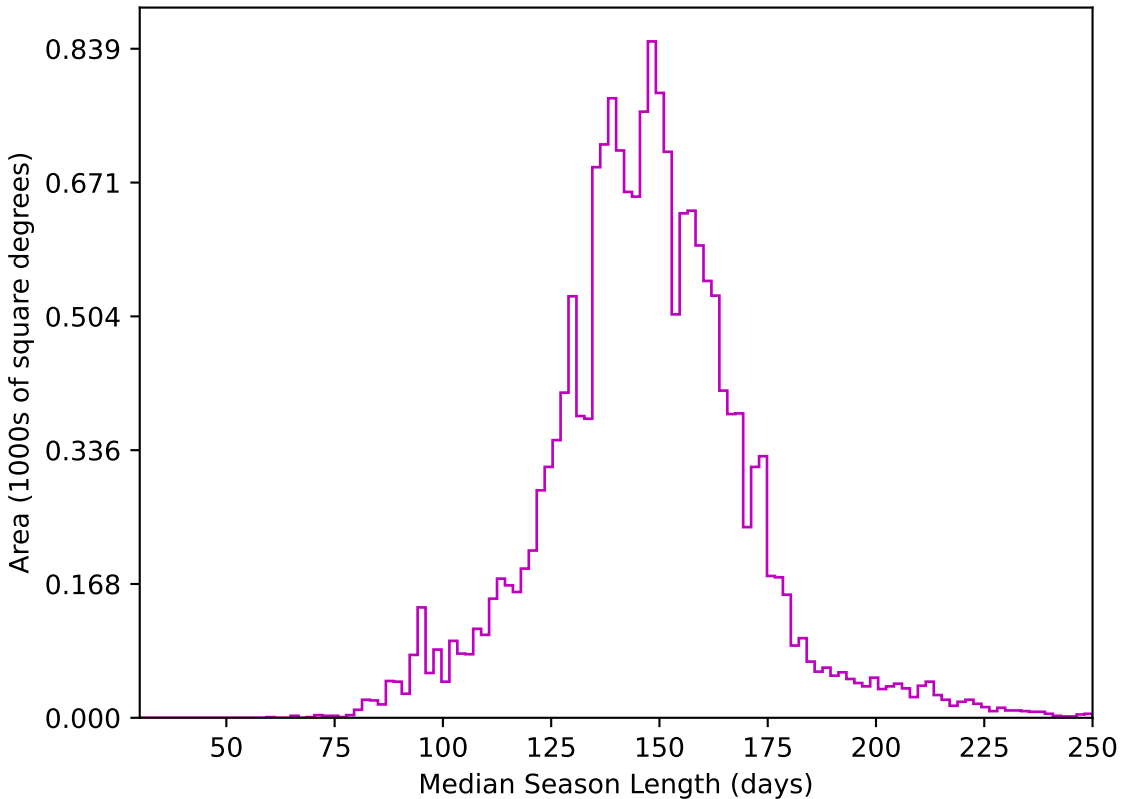
weather_cloudso4v3.4_10yrs WFD z band: Median Season Length
