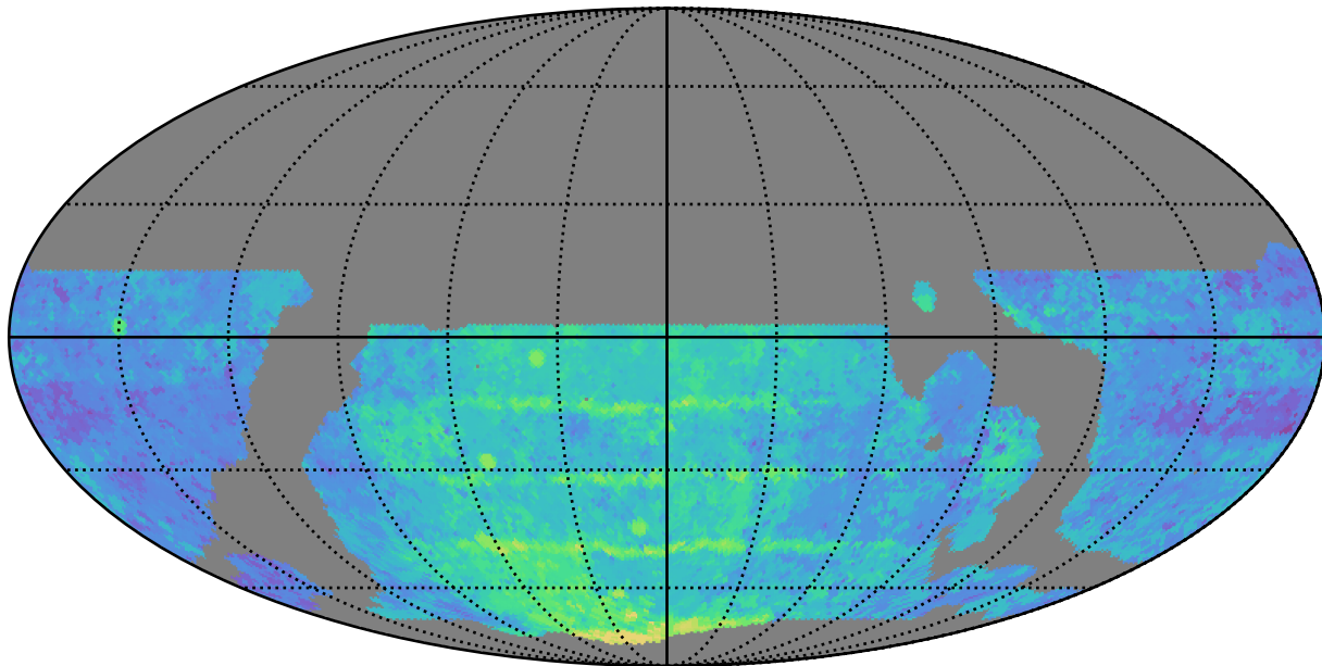
weather_cloudso4v3.4_10yrs WFD y band: Median Season Length
