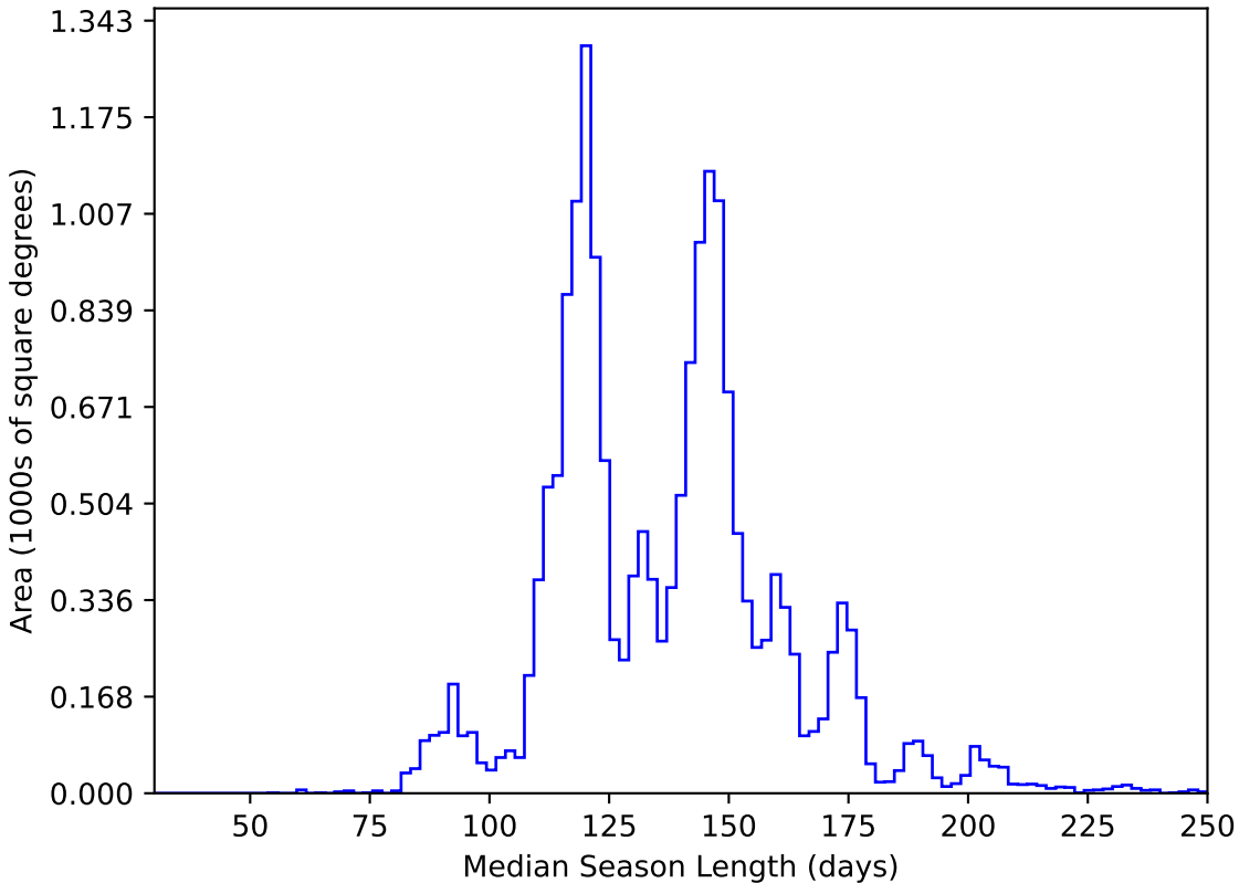
weather_cloudso4v3.4_10yrs WFD y band: Median Season Length
