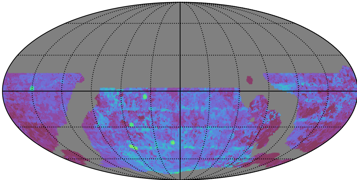
weather_cloudso4v3.4_10yrs WFD u band: Median Season Length
