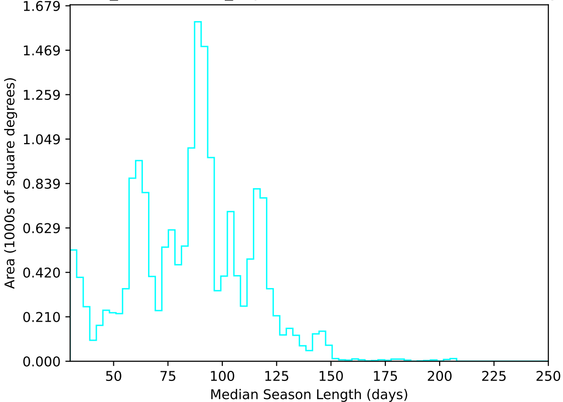
weather_cloudso4v3.4_10yrs WFD u band: Median Season Length
