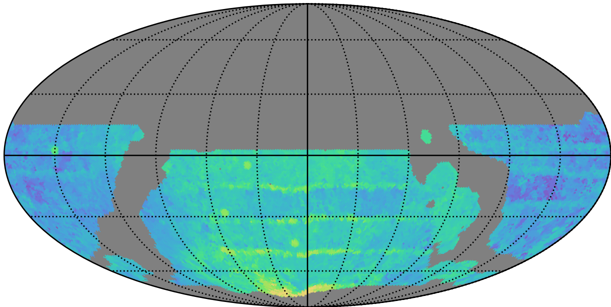
weather_cloudso4v3.4_10yrs WFD i band: Median Season Length
