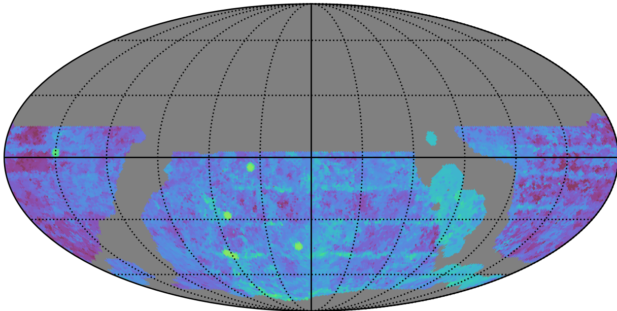
weather_cloudso4v3.4_10yrs WFD g band: Median Season Length
