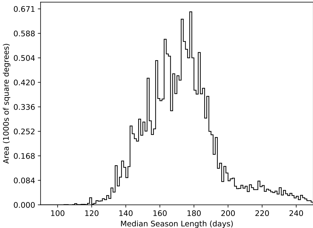
weather_cloudso4v3.4_10yrs WFD all bands: Median Season Length
