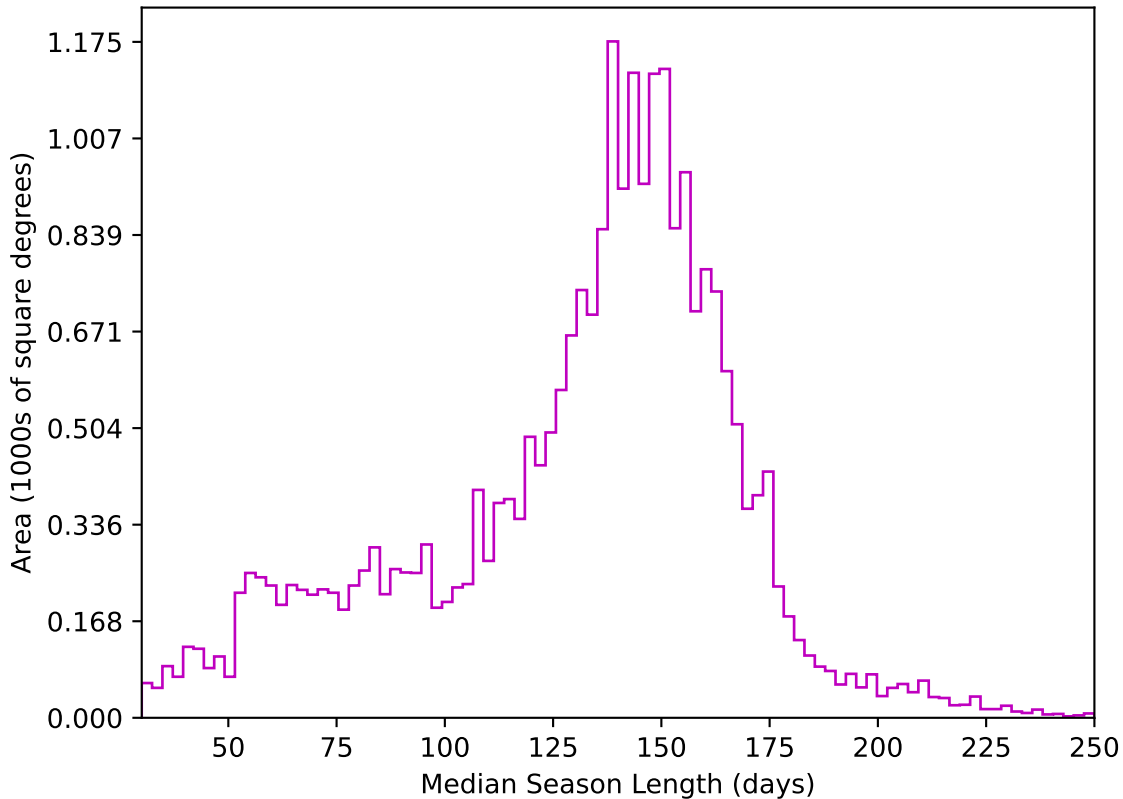
weather_cloudso4v3.4_10yrs All sky z band: Median Season Length
