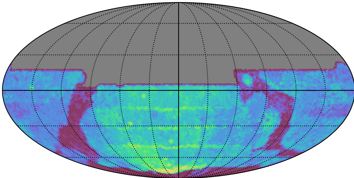
weather_cloudso4v3.4_10yrs All sky y band: Median Season Length
