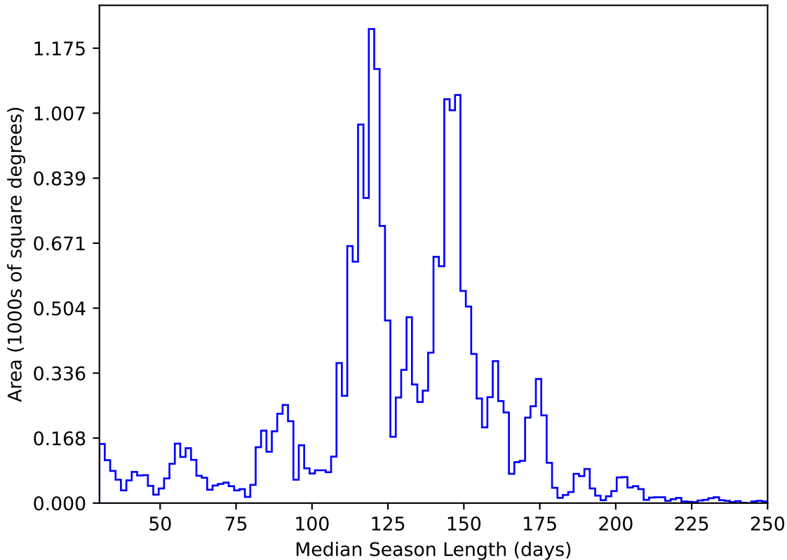
weather_cloudso4v3.4_10yrs All sky y band: Median Season Length
