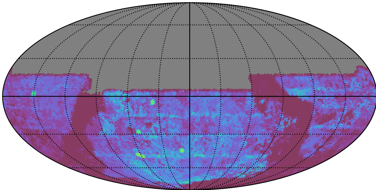
weather_cloudso4v3.4_10yrs All sky u band: Median Season Length
