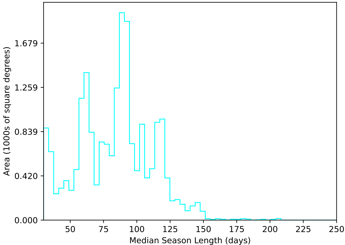
weather_cloudso4v3.4_10yrs All sky u band: Median Season Length
