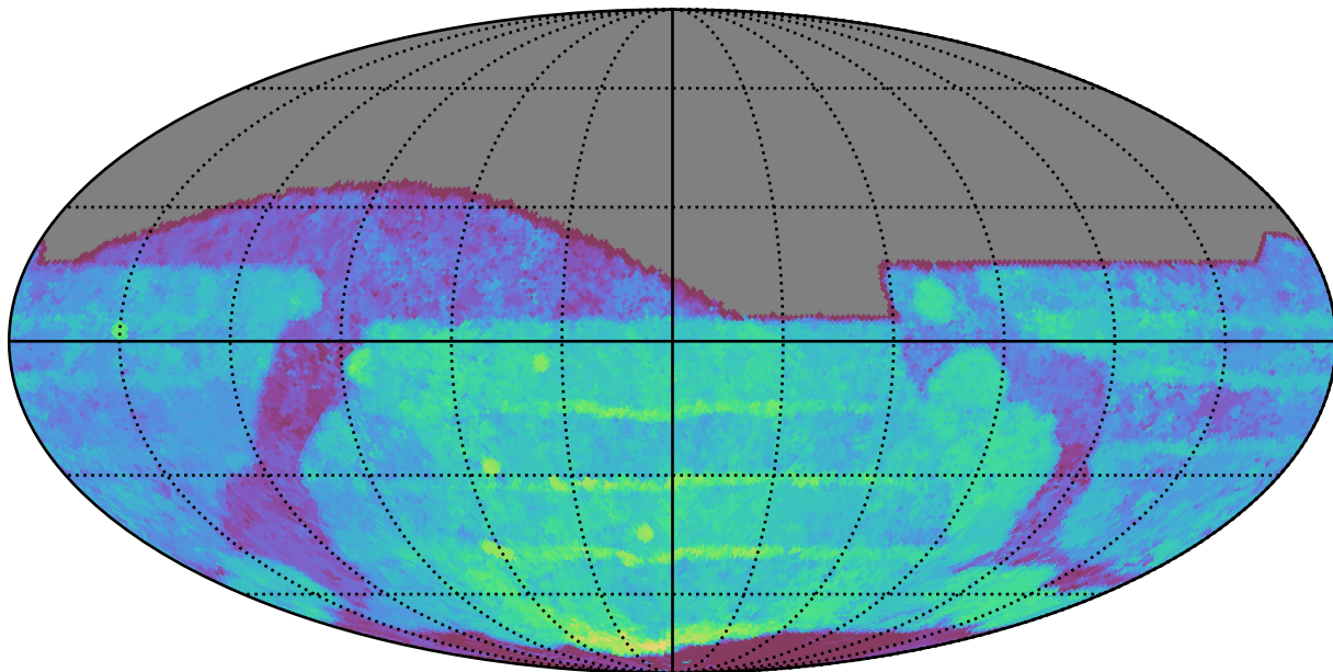
weather_cloudso4v3.4_10yrs All sky r band: Median Season Length
