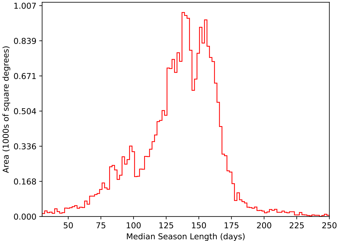
weather_cloudso4v3.4_10yrs All sky i band: Median Season Length
