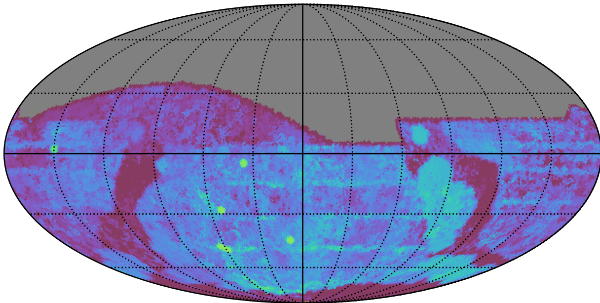
weather_cloudso4v3.4_10yrs All sky g band: Median Season Length
