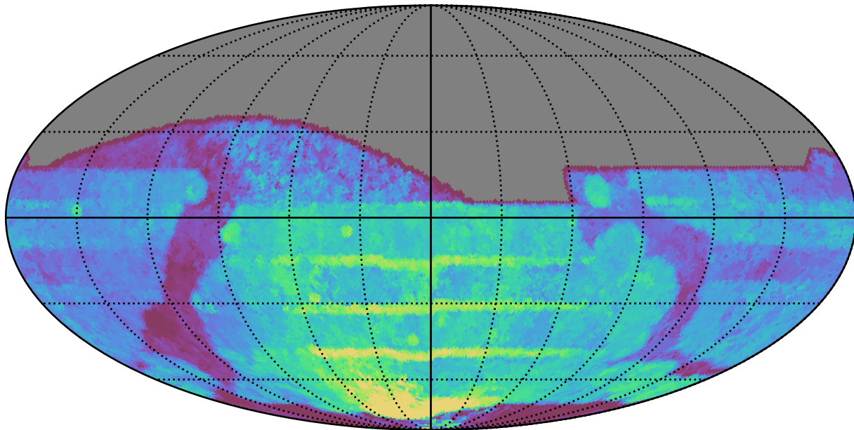
weather_cloudso4v3.4_10yrs All sky all bands: Median Season Length
