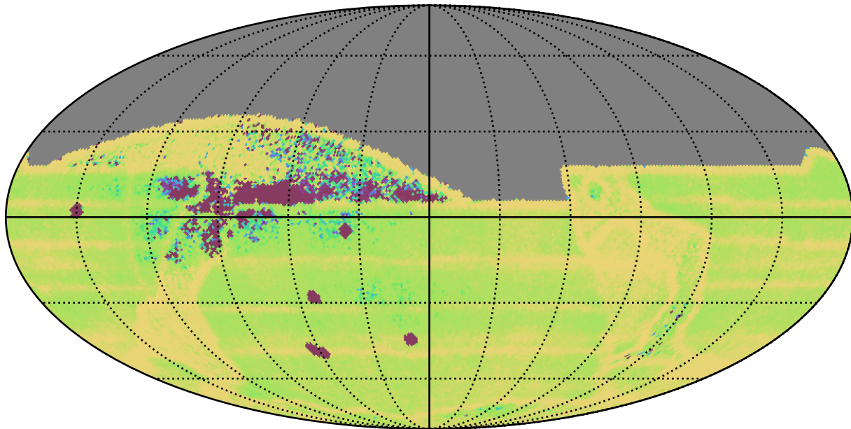
weather_cloudso4v3.4_10yrs All sky: Median Intra-Night Gap
