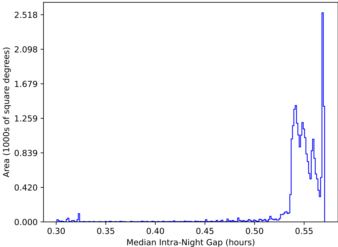
weather_cloudso4v3.4_10yrs All sky: Median Intra-Night Gap
