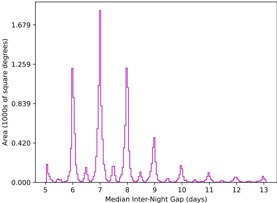
weather_cloudso4v3.4_10yrs WFD z band: Median Inter-Night Gap
