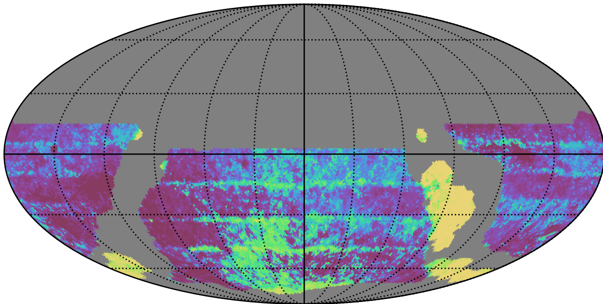
weather_cloudso4v3.4_10yrs WFD y band: Median Inter-Night Gap
