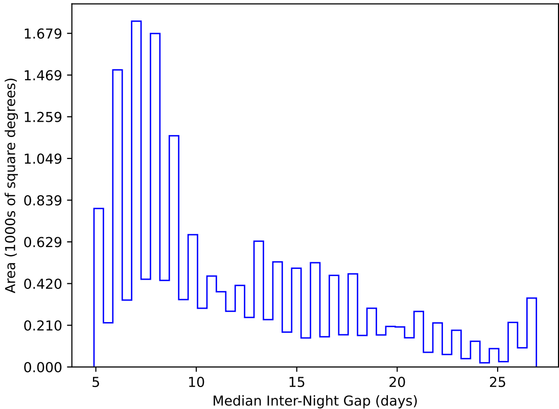
weather_cloudso4v3.4_10yrs WFD y band: Median Inter-Night Gap
