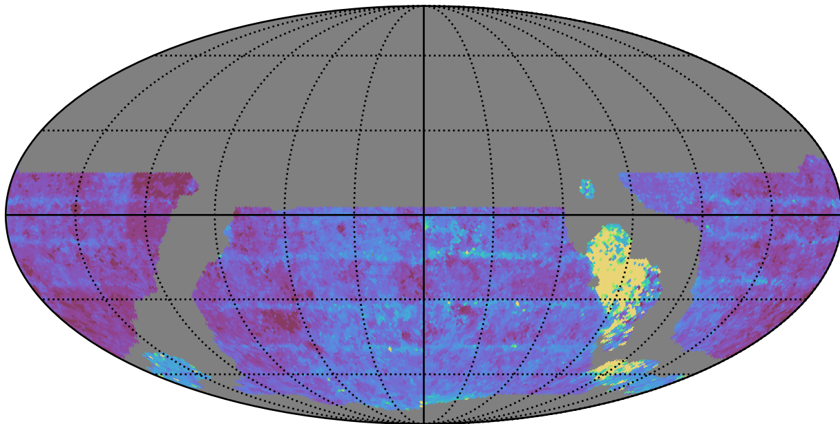
weather_cloudso4v3.4_10yrs WFD u band: Median Inter-Night Gap
