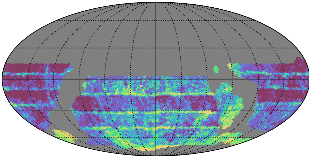
weather_cloudso4v3.4_10yrs WFD r band: Median Inter-Night Gap
