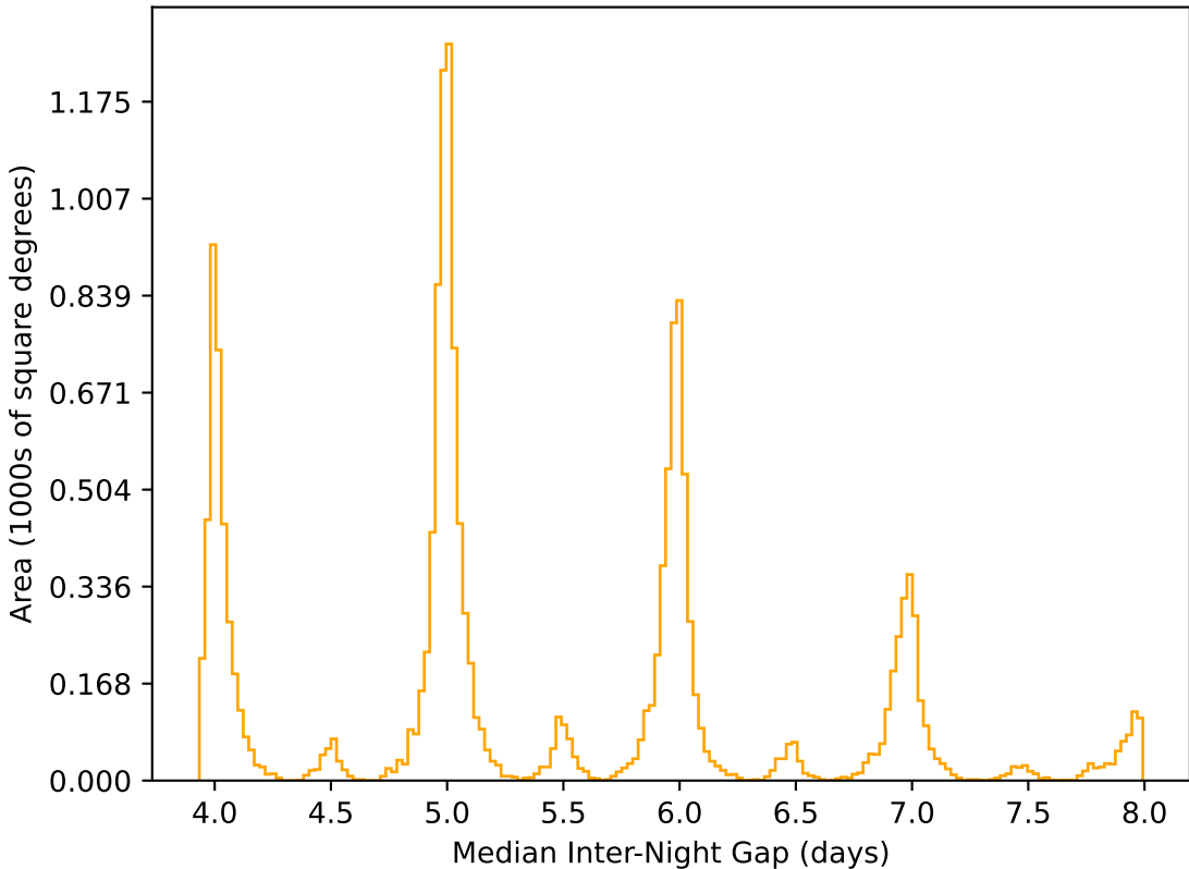
weather_cloudso4v3.4_10yrs WFD r band: Median Inter-Night Gap
