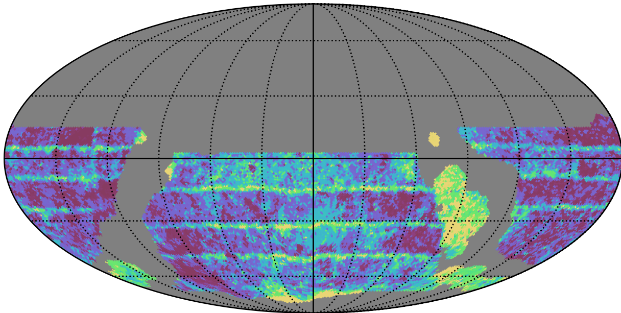
weather_cloudso4v3.4_10yrs WFD i band: Median Inter-Night Gap
