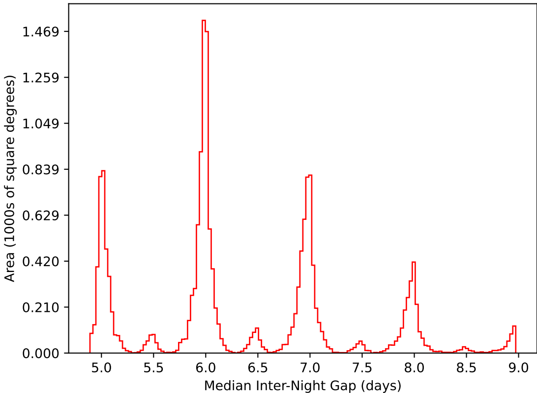
weather_cloudso4v3.4_10yrs WFD i band: Median Inter-Night Gap
