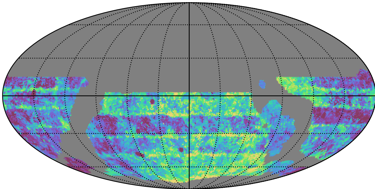
weather_cloudso4v3.4_10yrs WFD g band: Median Inter-Night Gap
