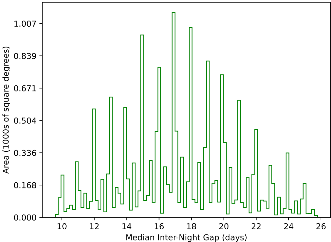
weather_cloudso4v3.4_10yrs WFD g band: Median Inter-Night Gap
