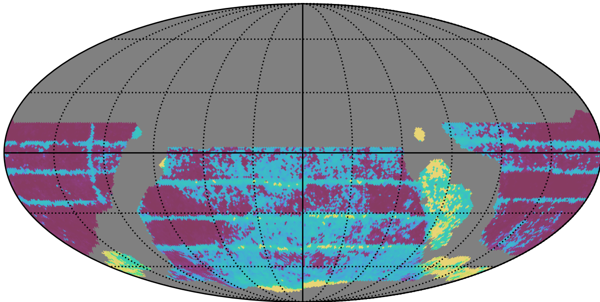
weather_cloudso4v3.4_10yrs WFD all bands: Median Inter-Night Gap
