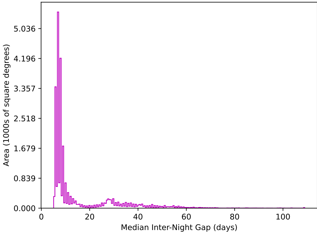
weather_cloudso4v3.4_10yrs All sky z band: Median Inter-Night Gap
