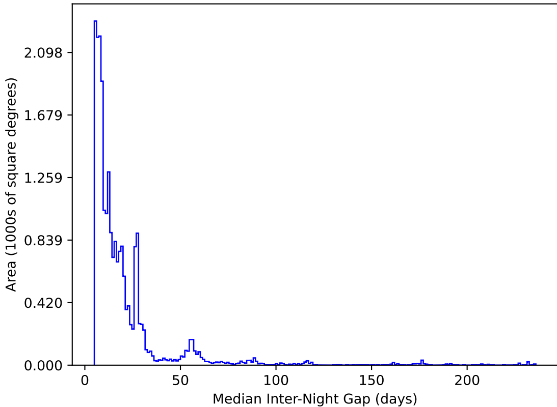
weather_cloudso4v3.4_10yrs All sky y band: Median Inter-Night Gap
