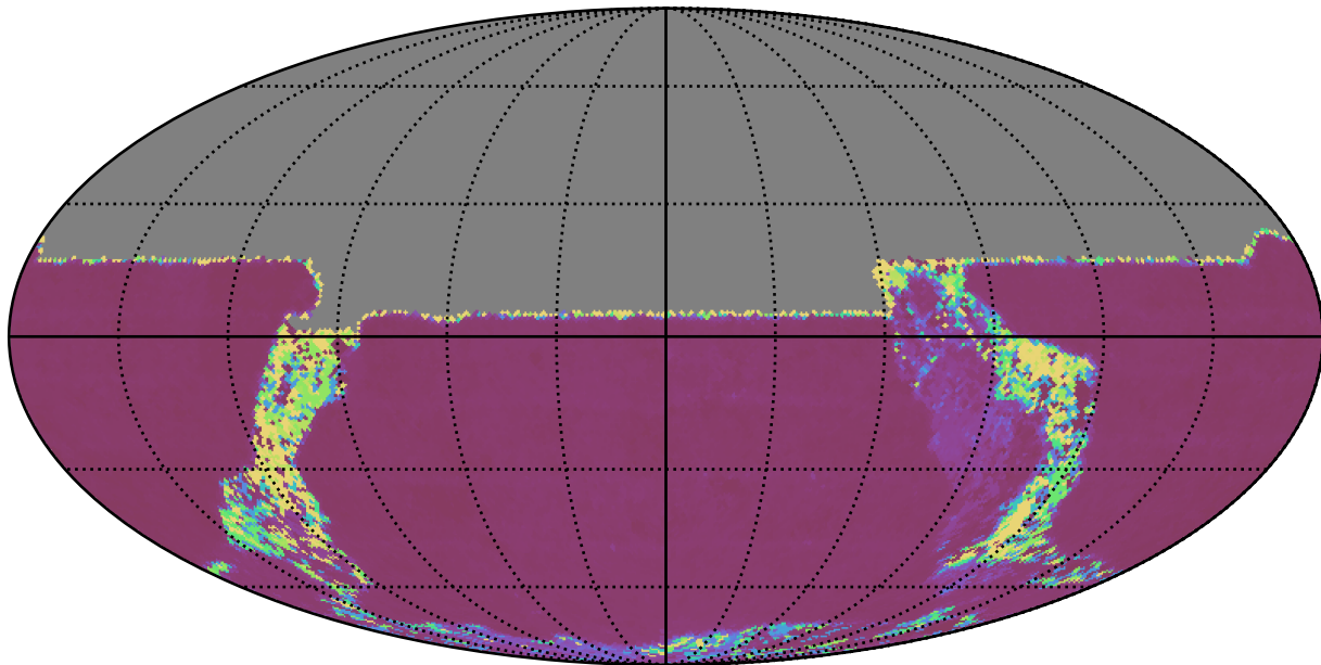
weather_cloudso4v3.4_10yrs All sky u band: Median Inter-Night Gap
