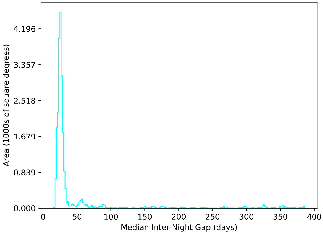
weather_cloudso4v3.4_10yrs All sky u band: Median Inter-Night Gap
