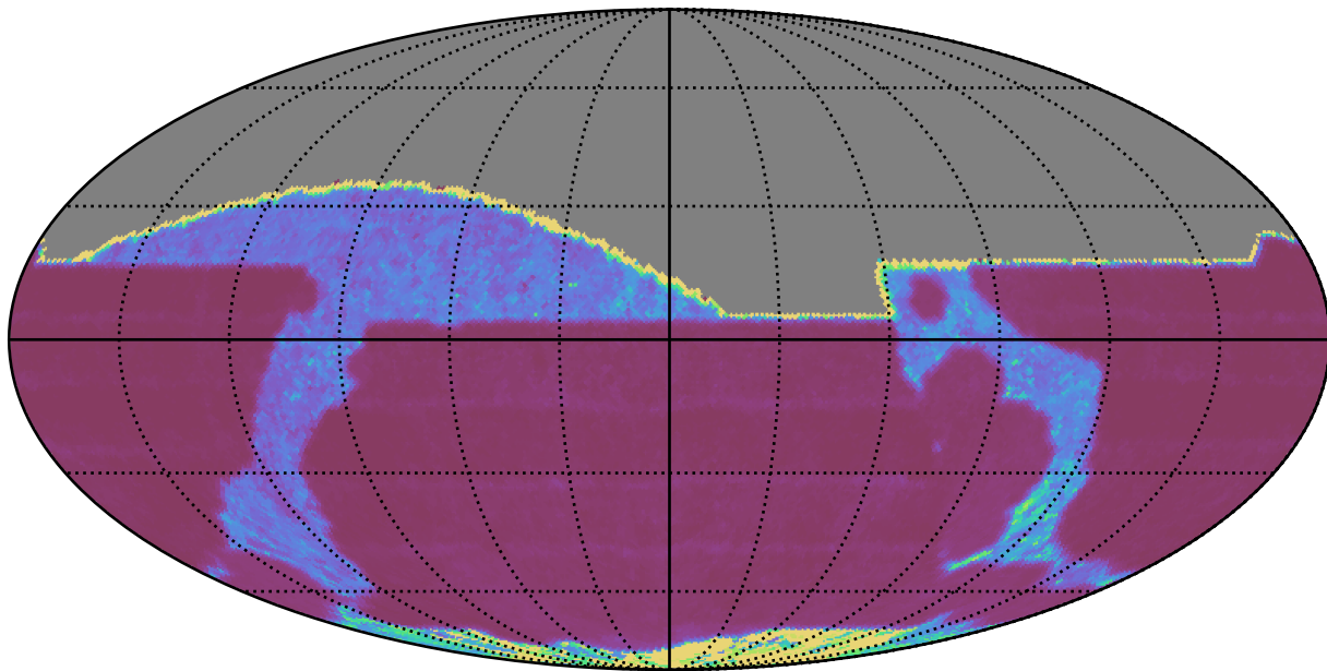
weather_cloudso4v3.4_10yrs All sky r band: Median Inter-Night Gap
