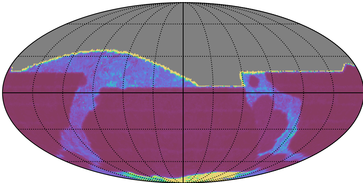
weather_cloudso4v3.4_10yrs All sky i band: Median Inter-Night Gap
