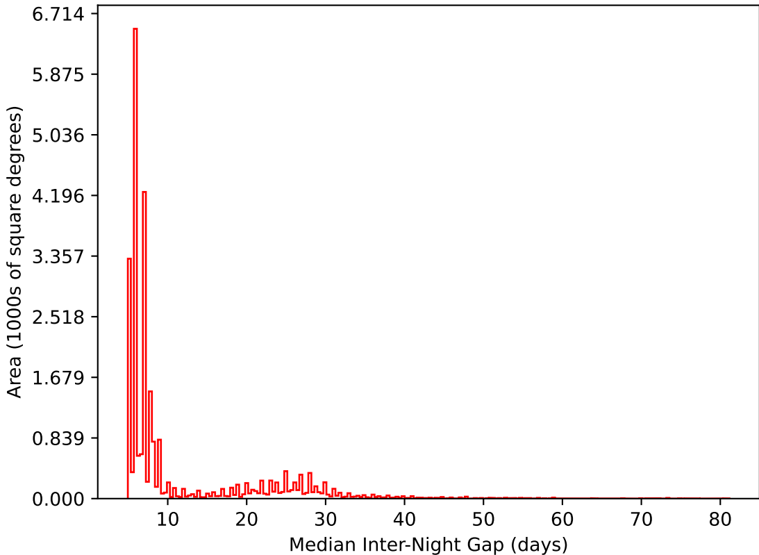
weather_cloudso4v3.4_10yrs All sky i band: Median Inter-Night Gap
